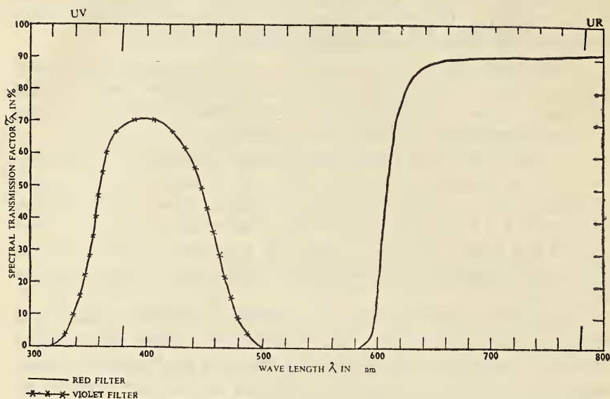
Fig. 1. Spectral transmission factors of red and violet filters.
